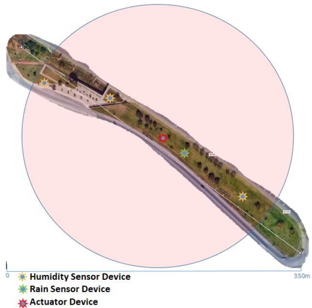
Fig. 2. SWAIS Prototype implementation example in Carlos Boto park in Lagoa. The red circle represents the range of the actuator device, and within it the several sensor devices.
